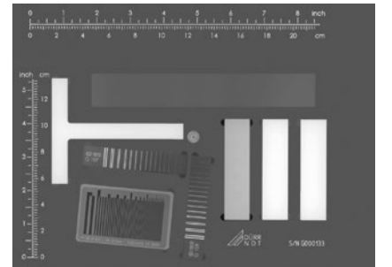
Test image of the DÜRR NDT CR-Phantom
